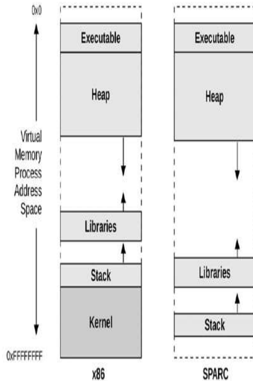
Figure 7.10 Example process virtual memory address space
