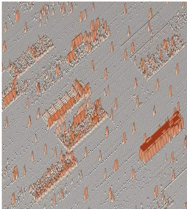
Figure 2.33 Wireframe surface plot: data center CPU utilization
