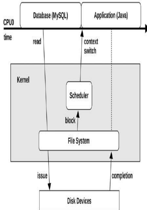
Figure 3.5 Asynchronous interrupt example
