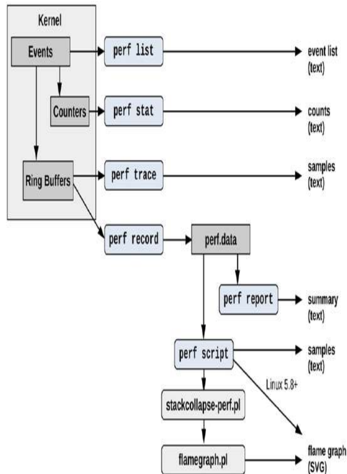
Figure 13.1 Commonly used perf subcommands
