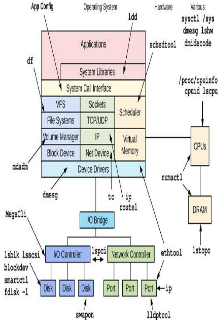
Figure 4.2 Linux static performance tuning tools
