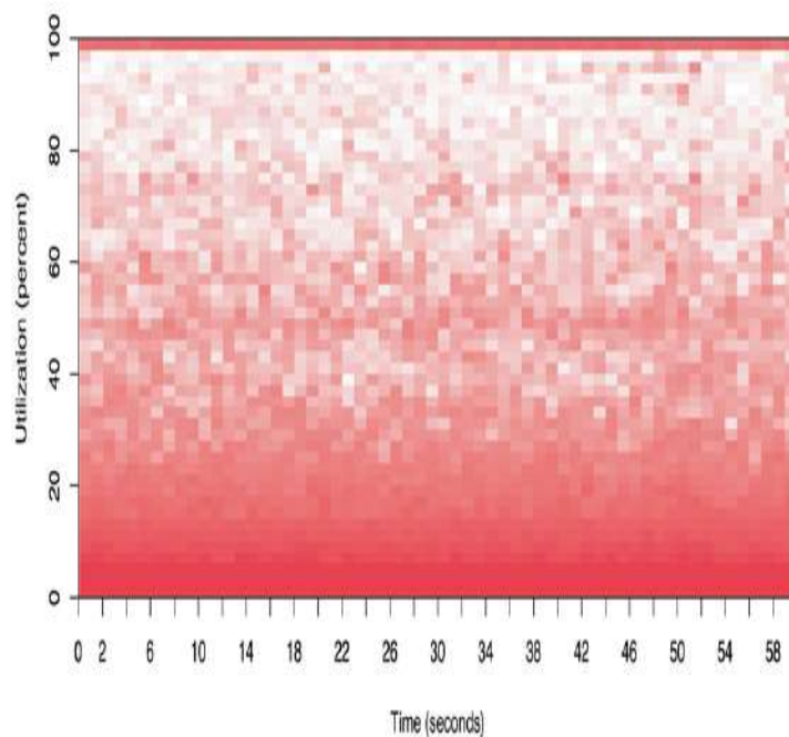
Figure 6.19 CPU utilization heat map, 5,312 CPUs
