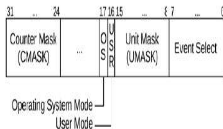
Figure 6.11 Example Intel performance event-select MSR
