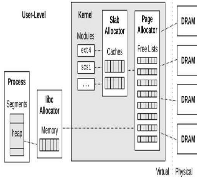
Figure 7.11 User- and kernel-level memory allocators
