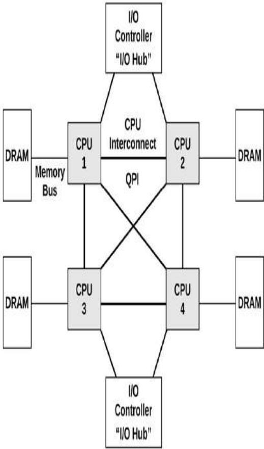
Figure 6.10 Example Intel QPI architecture, four-processor
