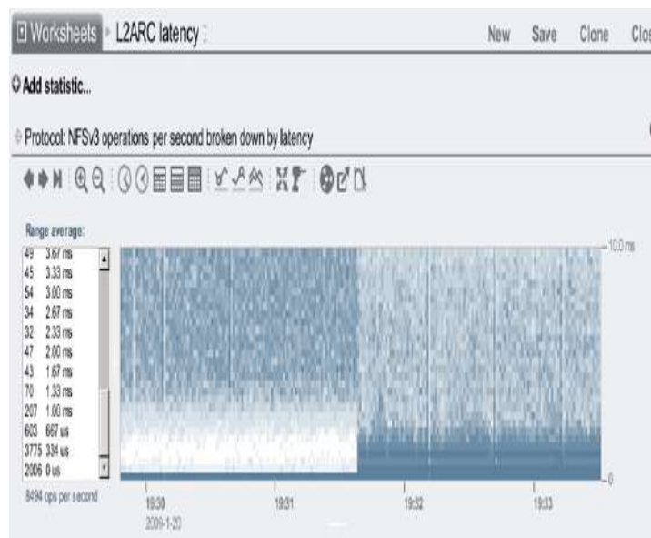
Figure 8.13 File system latency heat map
