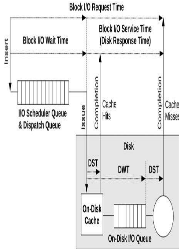
Figure 9.5 Kernel and disk time terminology
