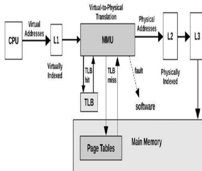
Figure 7.5 Memory management unit
