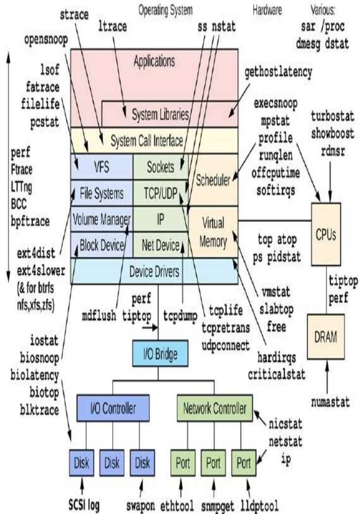
Figure 4.1 Linux workload observability tools
