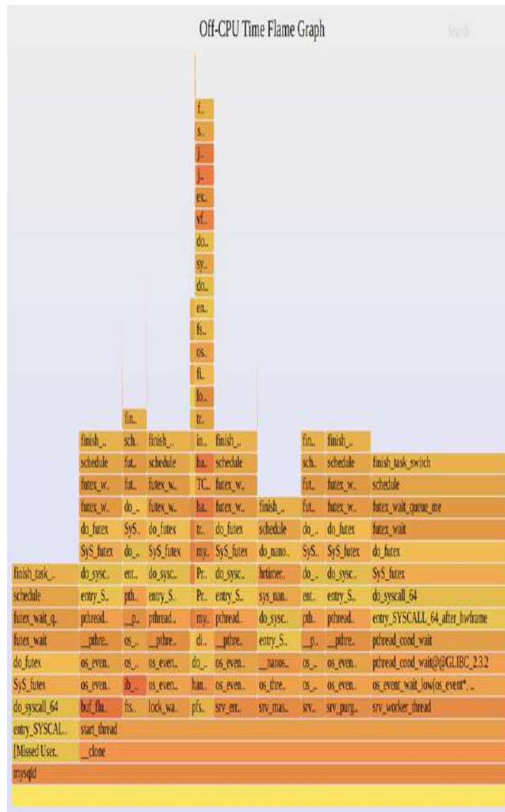
Figure 5.5 Off-CPU time flame graph, full
