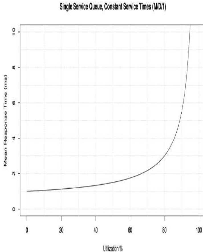
Figure 2.19 M/D/1 mean response time versus utilization
