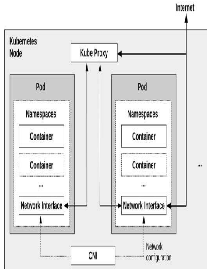
Figure 11.11 Kubernetes node
