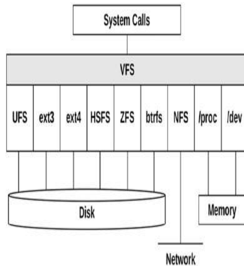
Figure 3.14 Virtual file system
