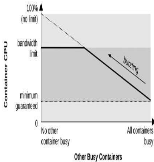
Figure 11.12 CPU shares and bandwidth
