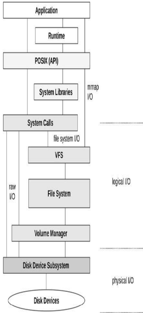
Figure 8.6 Generic file system I/O stack
