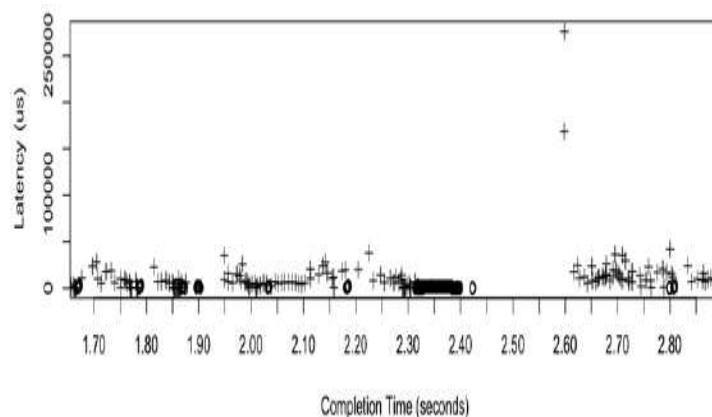
Figure 9.11 Scatter plot of disk read and write latency
