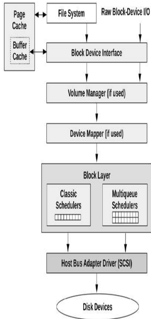
Figure 9.8 Linux I/O stack
