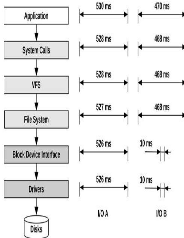
Figure 9.10 Stack latency analysis
