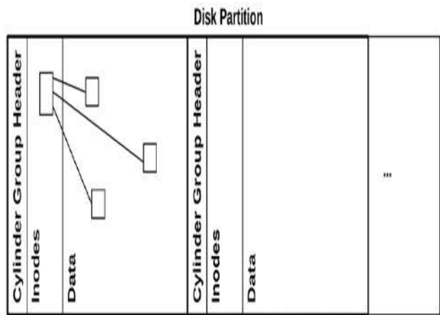
Figure 8.9 Cylinder groups
