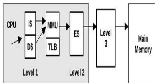
Figure 6.6 CPU cache hierarchy
