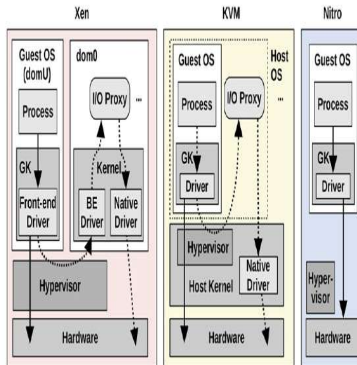
Figure 11.7 Xen, KVM, and Nitro I/O path
