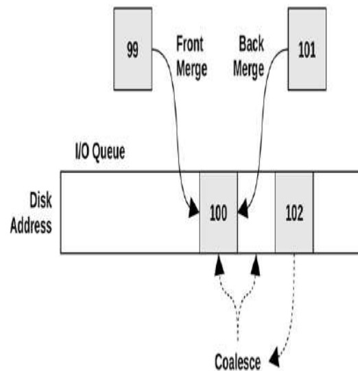
Figure 9.9 I/O merging types
