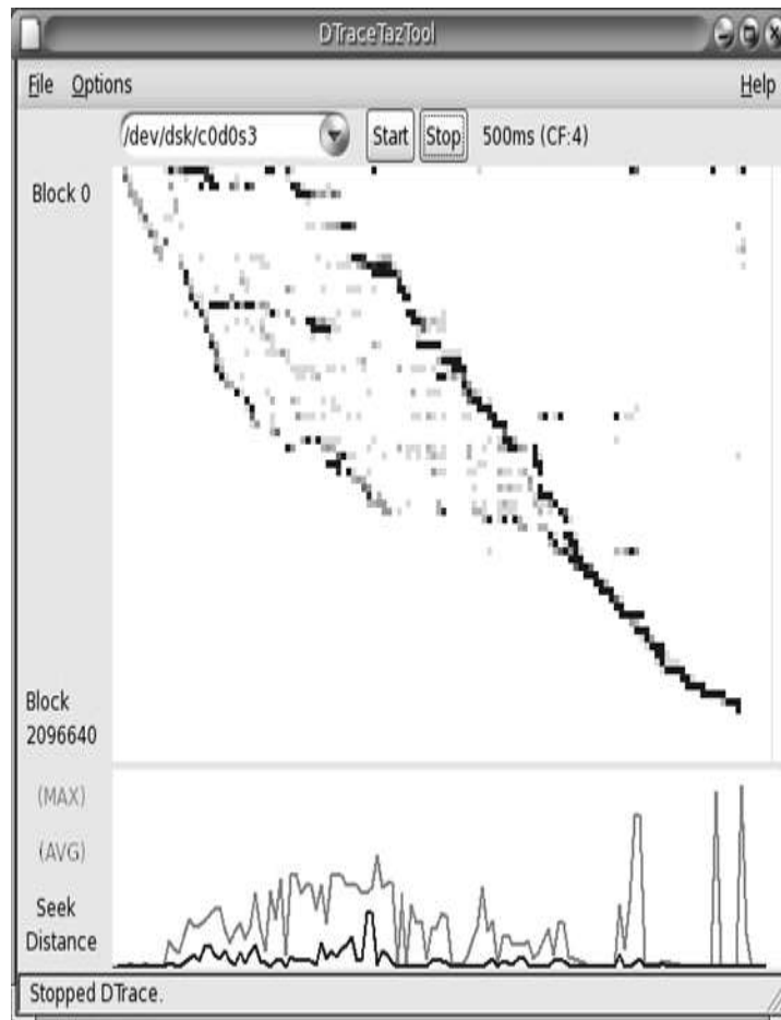
Figure 9.13 DTraceTazTool
