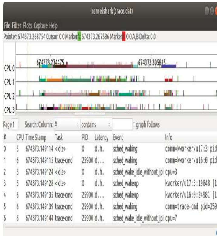
Figure 14.3 KernelShark
