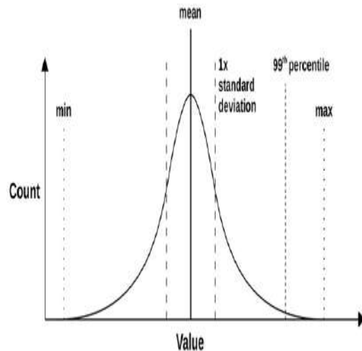
Figure 2.22 Statistical values
