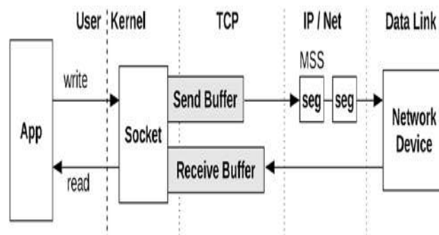
Figure 10.10 TCP send and receive buffers
