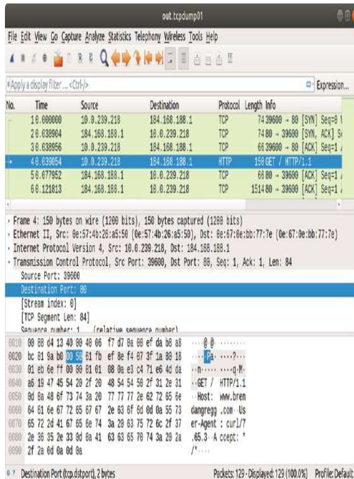
Figure 10.12 Wireshark screenshot
