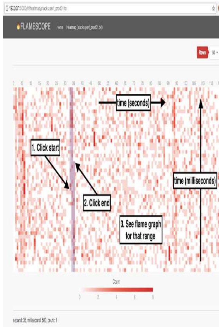
Figure 6.23 FlameScope
