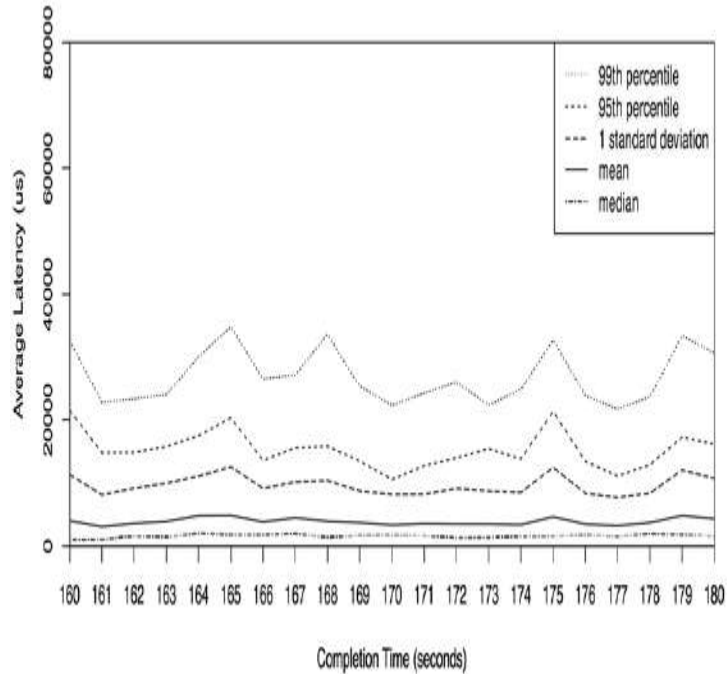
Figure 2.28 Median, mean, standard deviation, percentiles
