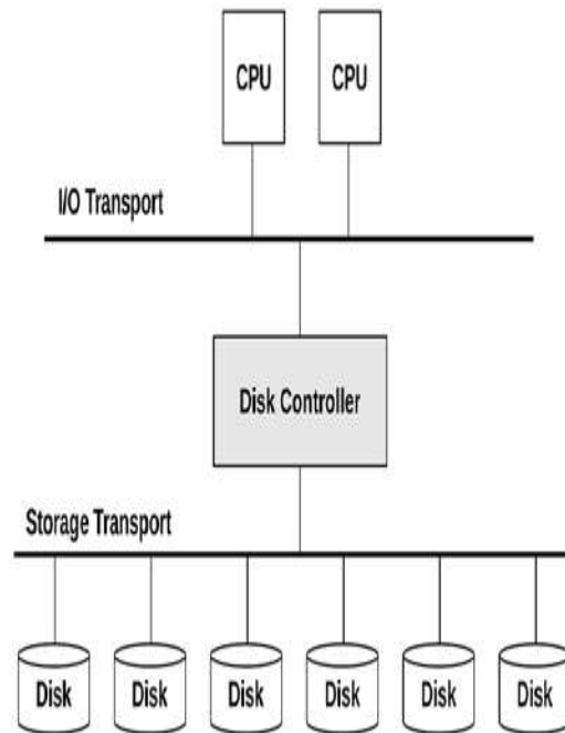
Figure 9.3 Simple disk controller and connected transports
