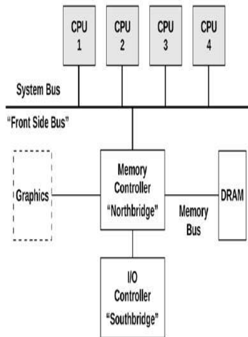
Figure 6.9 Example Intel front-side bus architecture, four-processor
