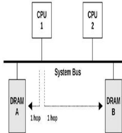
Figure 7.3 Example UMA main memory architecture, two-processor
