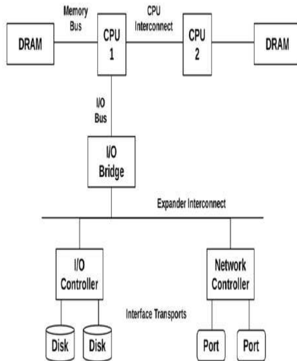
Figure 2.13 Example two-processor functional block diagram
