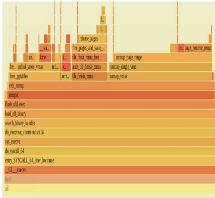
Figure 6.16 CPU flame graph excerpt
