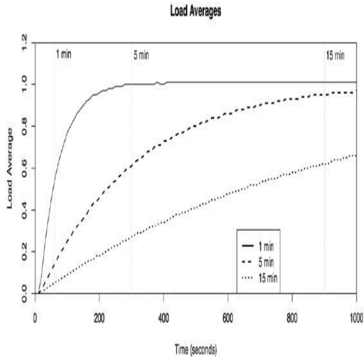
Figure 6.17 Exponentially damped load averages
