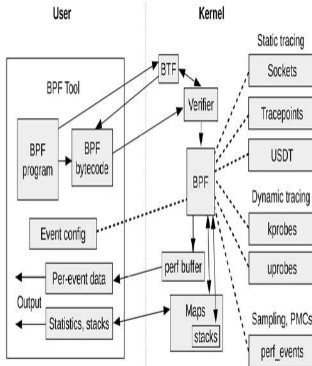
Figure 3.16 BPF components
