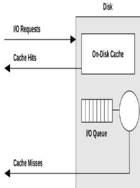
Figure 9.2 Simple disk with on-disk cache
