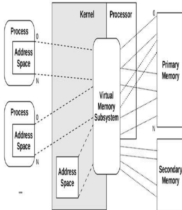
Figure 3.11 Virtual memory address spaces 13
