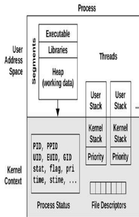
Figure 3.9 Process environment
