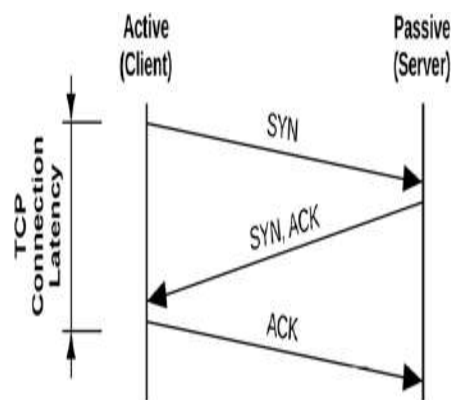
Figure 10.6 TCP three-way handshake
