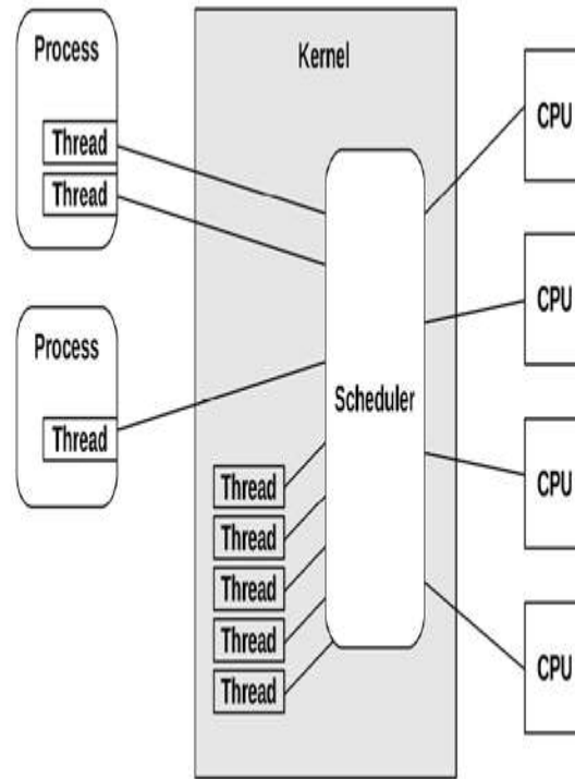
Figure 3.12 Kernel scheduler
