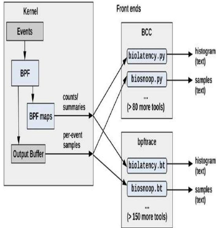
Figure 15.1 BPF tracing front ends
