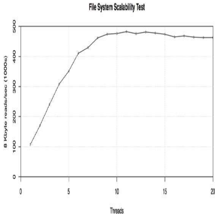
Figure 12.3 Ramping file system load
