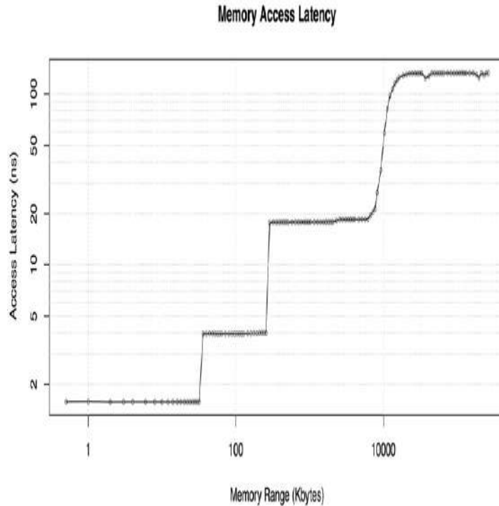
Figure 6.7 Memory access latency testing
