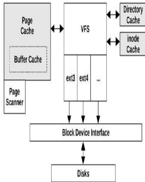
Figure 8.8 Linux file system caches
