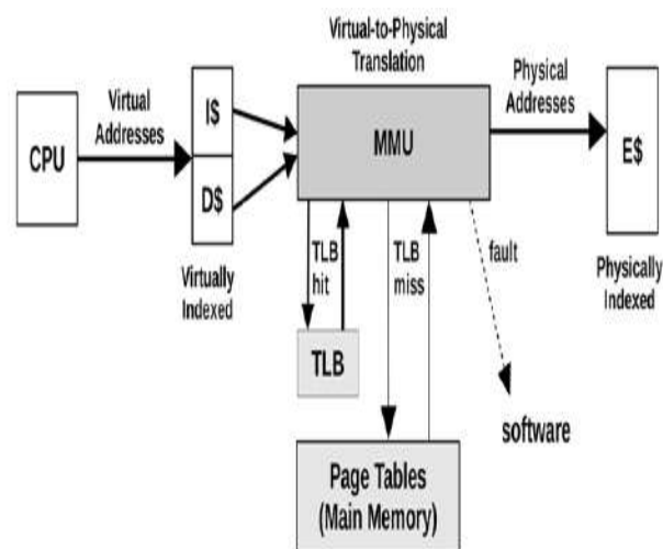
Figure 6.8 Memory management unit and CPU caches
