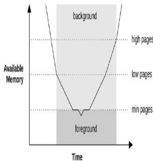
Figure 7.8 kswapd wake-ups and modes
