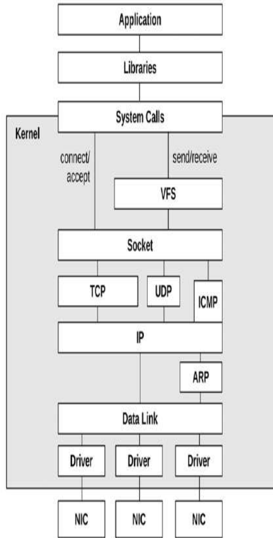
Figure 10.7 Generic network stack
