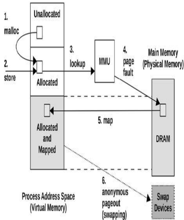
Figure 7.2 Page fault example
