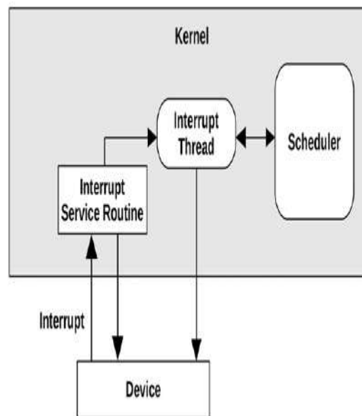
Figure 3.6 Interrupt processing
