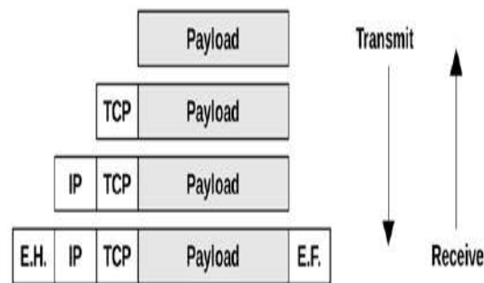
Figure 10.5 Network protocol encapsulation
