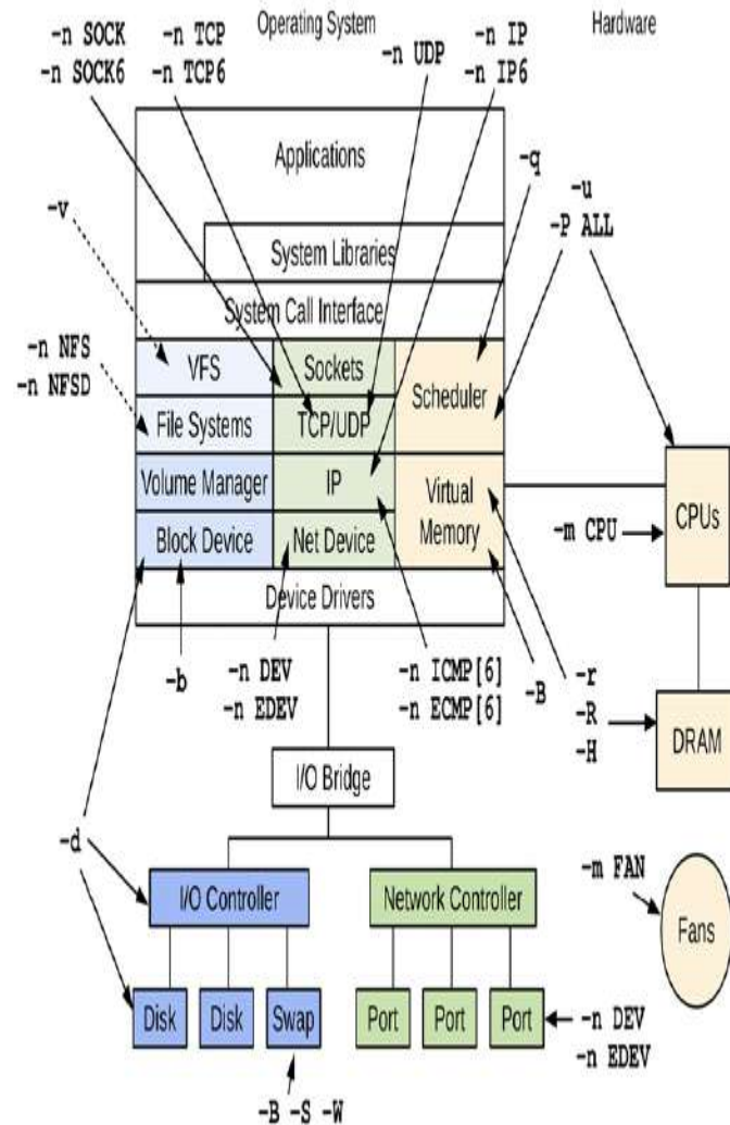
Figure 4.6 Linux sar(1) observability
