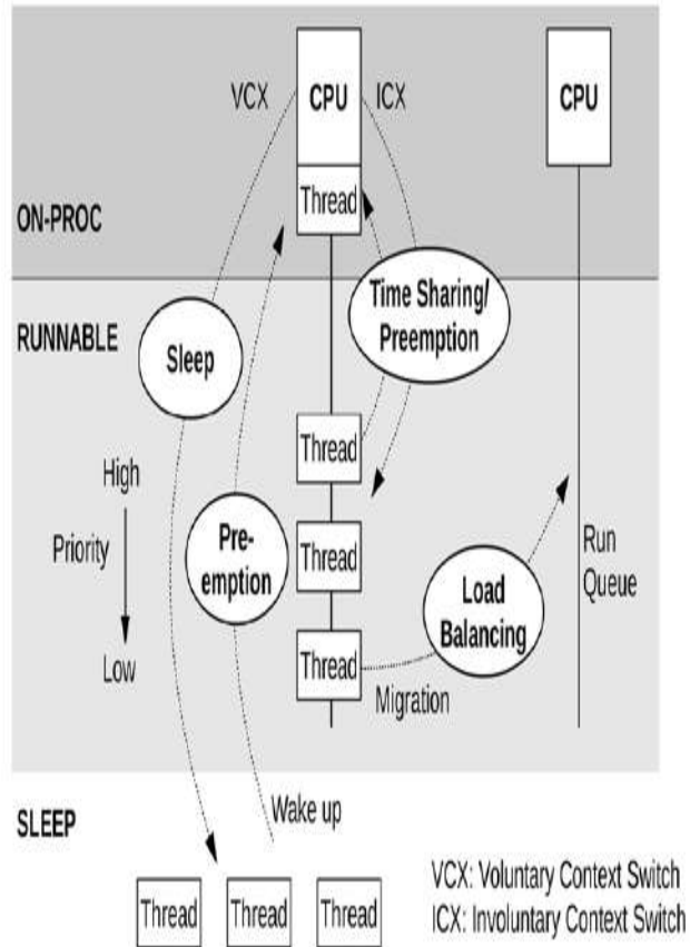
Figure 6.12 Kernel CPU scheduler functions
