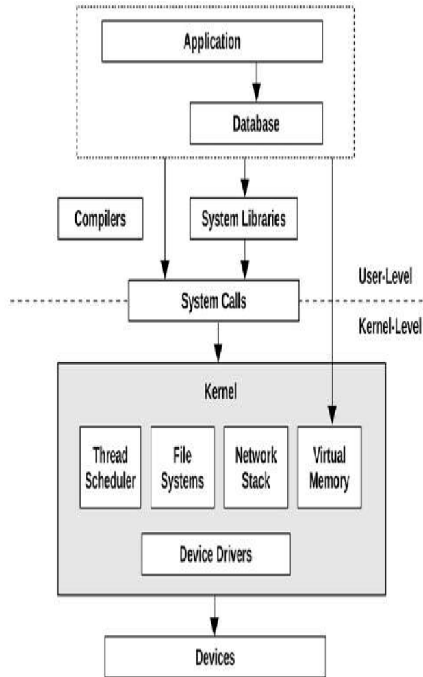
Figure 1.1 Generic system software stack
