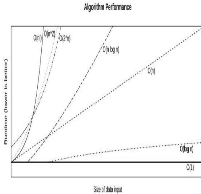
Figure 5.1 Runtime versus input size for different algorithms
