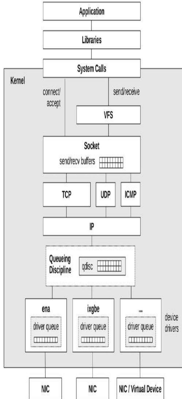
Figure 10.8 Linux network stack
